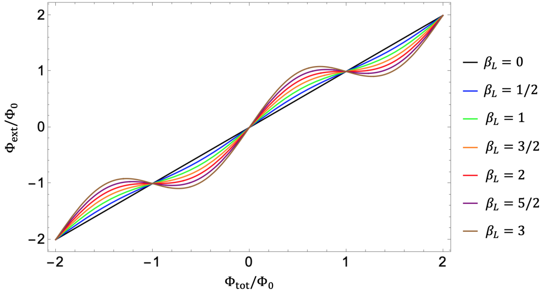
Figure 3.4: Total versus externally applied flux for a SQUID with different geometrical inductances, Eq. (3.42). When \beta_L > 2 (purple and brown curves) some values of \Phi_{\text{ext}} become associated with multiple values of \Phi_{\text{tot}} , and the SQUID becomes hysteretic.
