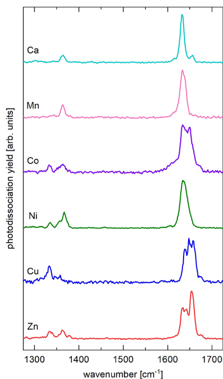
Figure 2. Experimental IR spectra of [\text{M}(\text{II})\cdot\text{EDTA}]^{2-}\cdot\text{N}_2 complexes in the fingerprint region (from top to bottom: \text{M} = \text{Ca} , \text{Mn} , \text{Co} , \text{Ni} , \text{Cu} , and \text{Zn} ; metal identity given in each trace). Data for \text{M} = \text{Ca} taken from ref 7.
