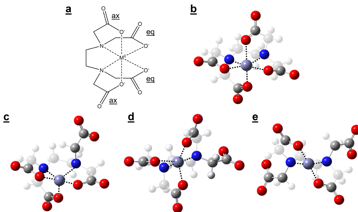
Figure 1. Structure of EDTA complexes with metal dications. (a) [M(\text{II})\cdot\text{EDTA}]^{2-} line drawing; equatorial and axial ligands are labeled “eq” and “ax”, respectively. (b–e) Calculated ball-and-bond-type structures of [M(\text{II})\cdot\text{EDTA}]^{2-} complexes in hexa- (b), penta- (c, d), and tetra-coordinated (e) geometries using M = \text{Zn} as an example. Pentacoordinated structures can have an axial (c) or equatorial ligand (d) detached from the metal center. The metal environment in the tetra-coordinated structures (e) is approximately tetrahedral, making such distinctions less useful. Carbon atoms are shown in gray, hydrogen in white, nitrogen in blue, oxygen in red, and the central metal atom in blue-gray. Dotted lines show the coordination of the metal atom. The parts of the EDTA molecule that are not part of the binding pocket are shown in lighter gray tones.
