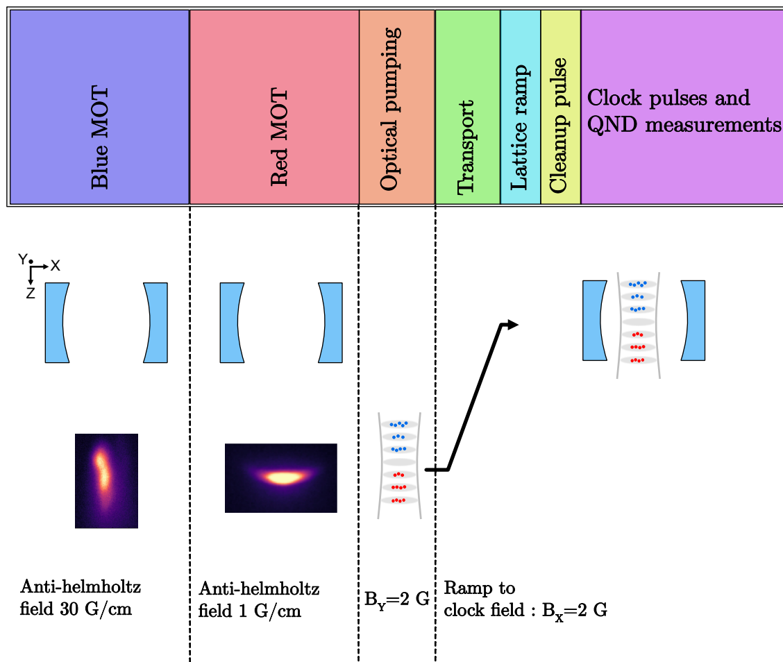
Figure 5.7: The top panel shows the experimental sequence roughly laid out in time. Below we graphically indicate the location of the MOTs, and the subsequent loading of the lattice and transport into the cavity. We also note the magnitude and direction of the relevant magnetic field for each step.
