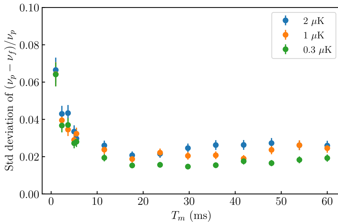
Figure 4.3: Simulations of cavity frequency shift noise arising from thermal atomic motion. With a fixed separation time between measurements of 10 ms, we predict fluctuations in the shifted cavity frequency on the percent level. Both low atomic temperatures and longer measurement time T_m are critical for minimizing this effect.
