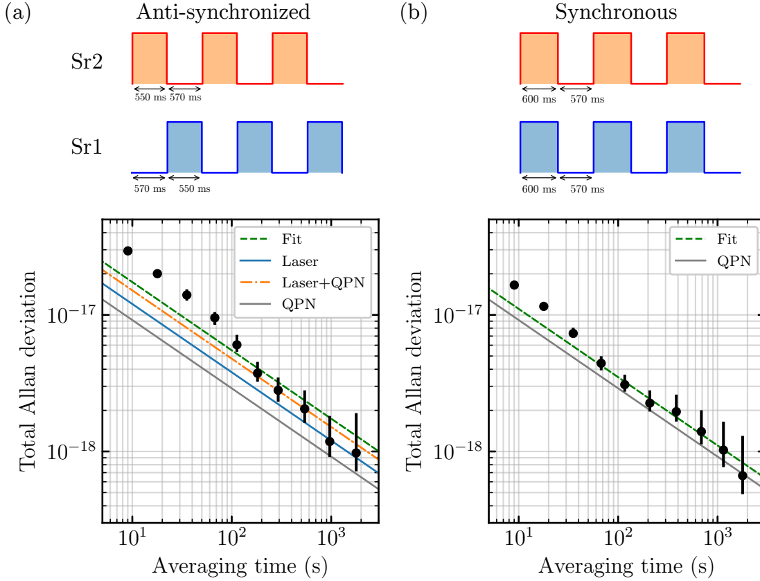
Figure 3.2: (a) Anti-synchronized clock comparison between Sr1 and Sr2. The solid gray line is the calculated QPN, blue line is calculated Dick effect, orange dashed-dotted is the quadrature sum of QPN and the Dick effect laser noise, and the dashed green line is the fitted stability, giving 5.5 \times 10^{-17}/\sqrt{\tau} . (b) Synchronous comparison, showing a single clock stability of 3.5 \times 10^{-17}/\sqrt{\tau} .
