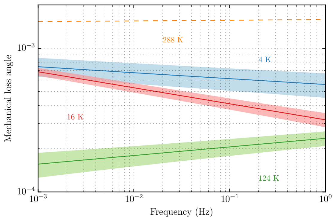
Figure 2.14: Frequency-dependent mechanical loss angle for the SiO 2 /Ta 2 O 5 coatings at different operating temperature. The shaded bands indicate the 1σ uncertainty.
