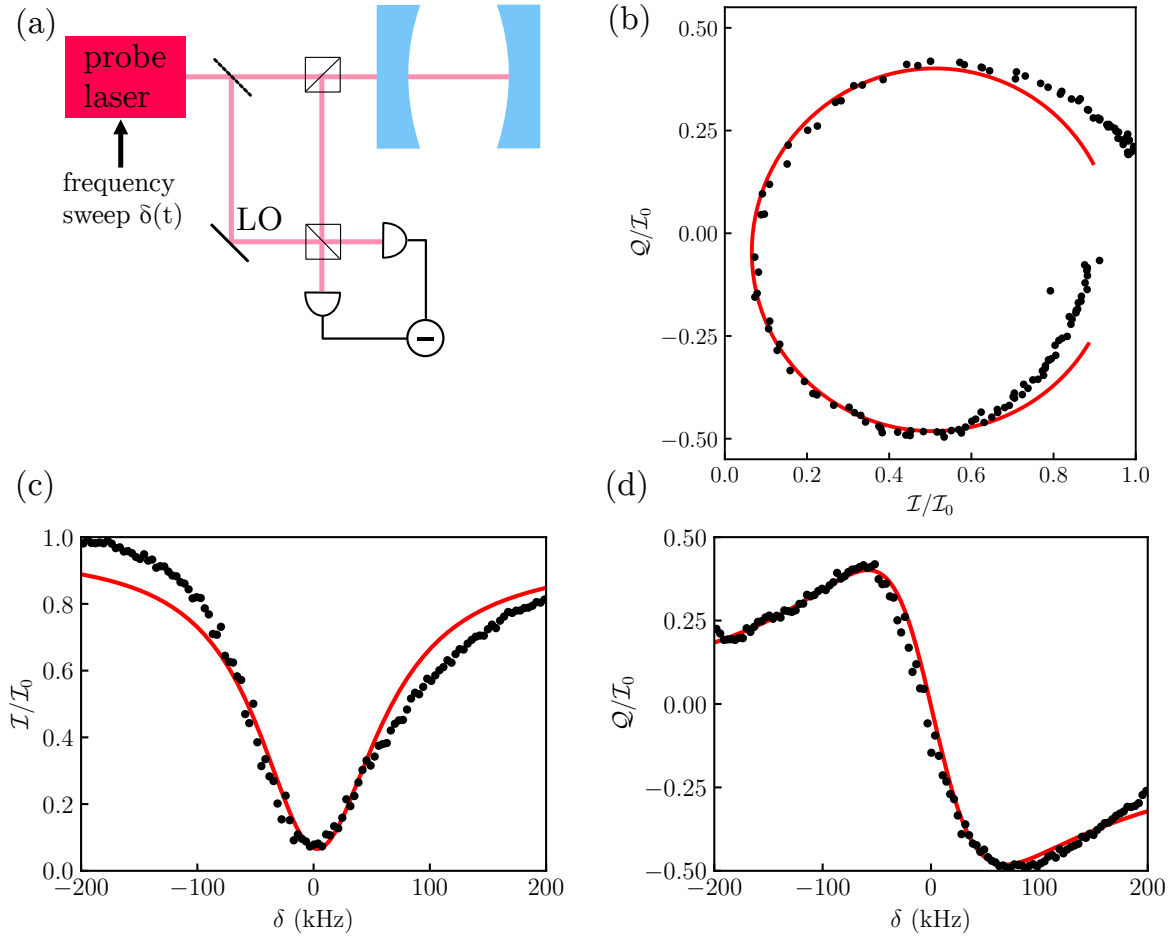
Figure 4.1: (a) Schematic of the detection scheme, where laser light is split into a probe path and LO path, and these are combined on a beamsplitter. (b) By sweeping the probe laser across resonance we can map out the \mathcal{I} - \mathcal{Q} response of the cavity response. (c) Normalized \mathcal{I} quadrature. (d) Normalized \mathcal{Q} quadrature.
