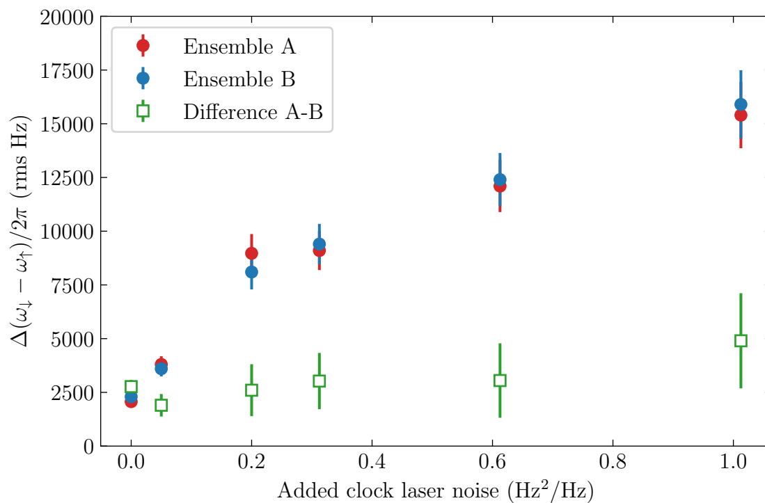
Figure 7.5: Measured cavity shift noise with artificial white frequency noise imposed on the clock laser. Each ensemble (red and blue circles) becomes noisier as the magnitude of the added noise is increased, but taking the difference (open green squares) gives a 10 dB common mode noise reduction factor.
