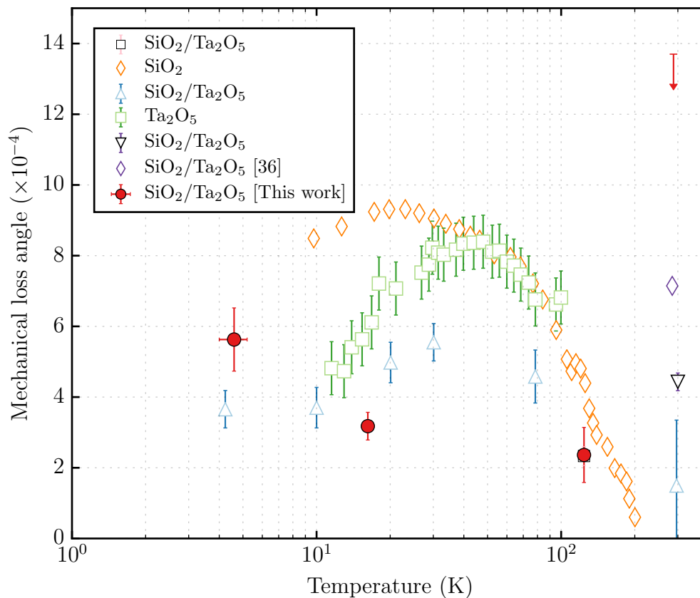
Figure 2.15: Mechanical loss of the individual coating constituents ( \text{SiO}_2 , \text{Ta}_2\text{O}_5 ), and \text{SiO}_2/\text{Ta}_2\text{O}_5 coatings measured by ringdown (orange diamonds [75], blue triangles [76], green squares [77]). Other direct measurements are also included (black triangle [78], open black square [25], and purple diamond [79]). Our results from direct CTN measurements are shown as the red circles and the red arrow.
