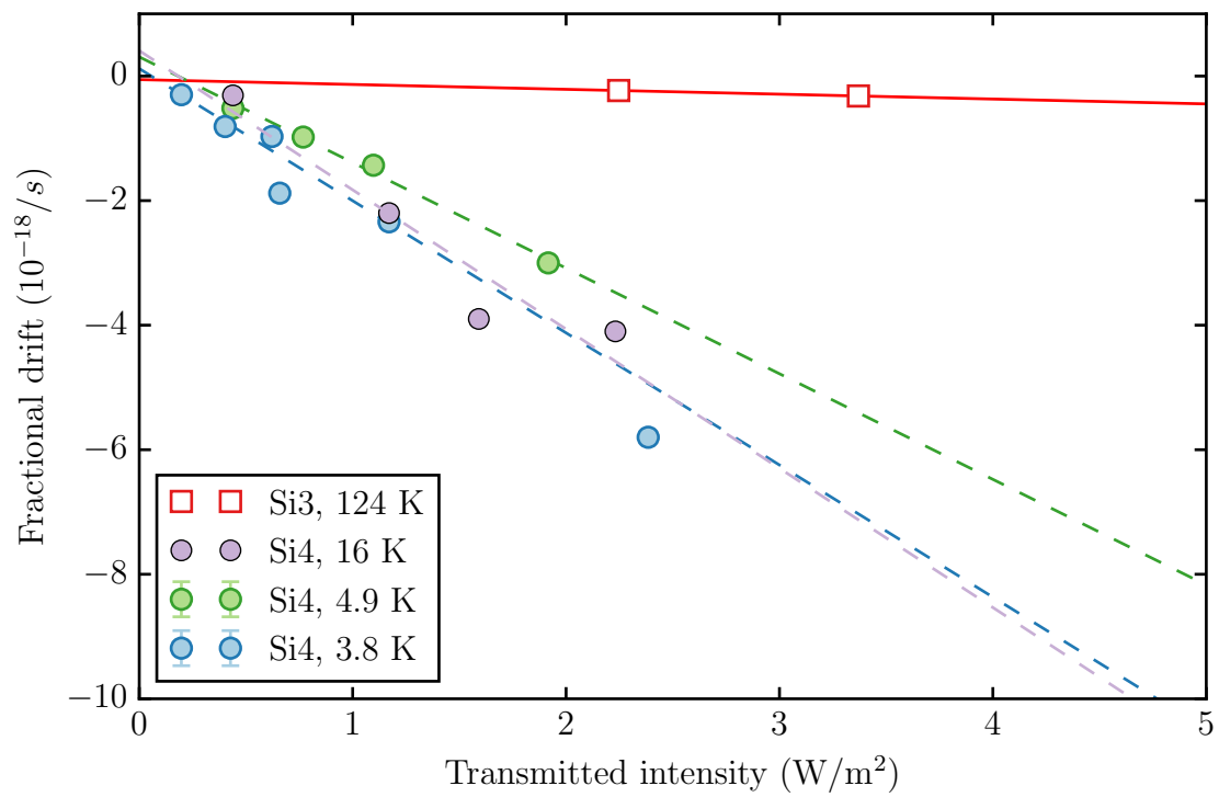
Figure 2.11: Fractional frequency drift in units of 10^{-18} for Si4 at different operating temperature. The Si3 drift versus intensity is shown as the open red squares, exhibiting a far smaller sensitivity to optical power.
