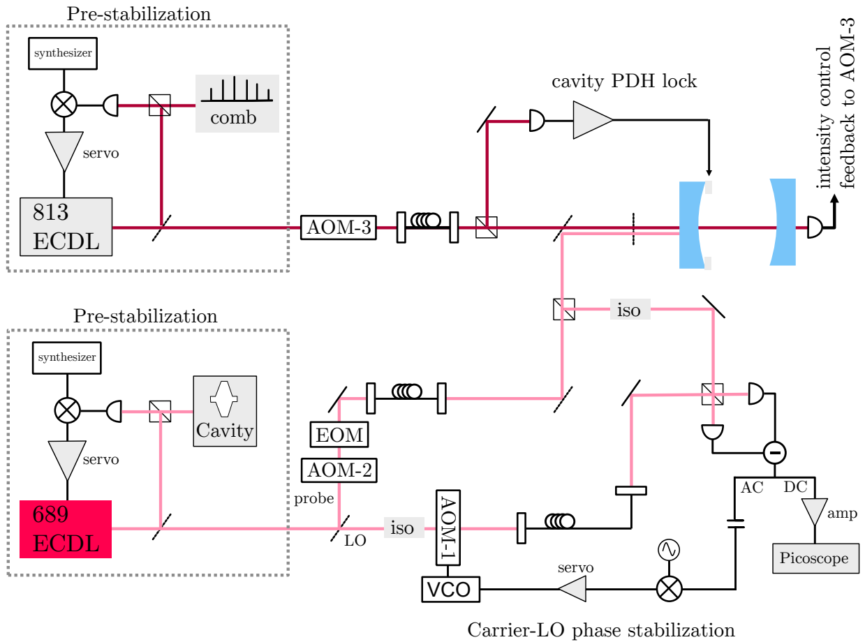
Figure 5.12: The optics layout and stabilization scheme of the cavity QED setup. The 813nm laser is pre-stabilized, and the cavity is locked to that pre-stabilized laser via the cavity PDH lock. The 689nm laser is pre-stabilized to the red cavity system. The 689 ECDL is split into the LO and probe path. The leakage light from the cavity is detected via homodyne detection.
