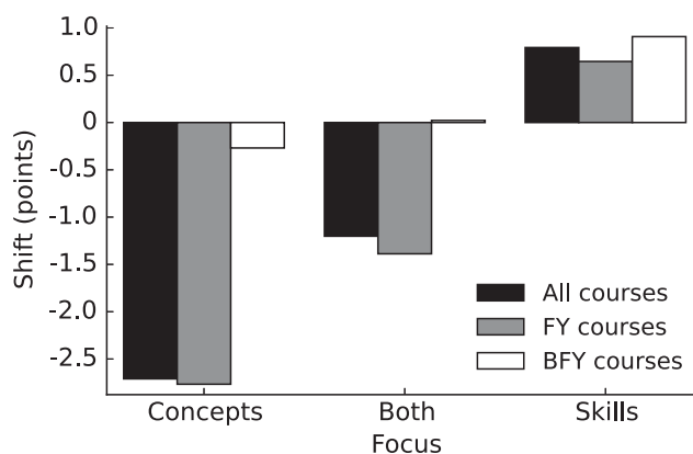
FIG. 1. Visual representation of pre- to postinstruction shifts in E-CLASS scores from all courses in the data set, as well as for the FY and BFY courses individually. Differences in the pre- and postinstruction score distributions are statistically significant in all cases except for those of the BFY students in the concepts-focused and both-focused courses.
