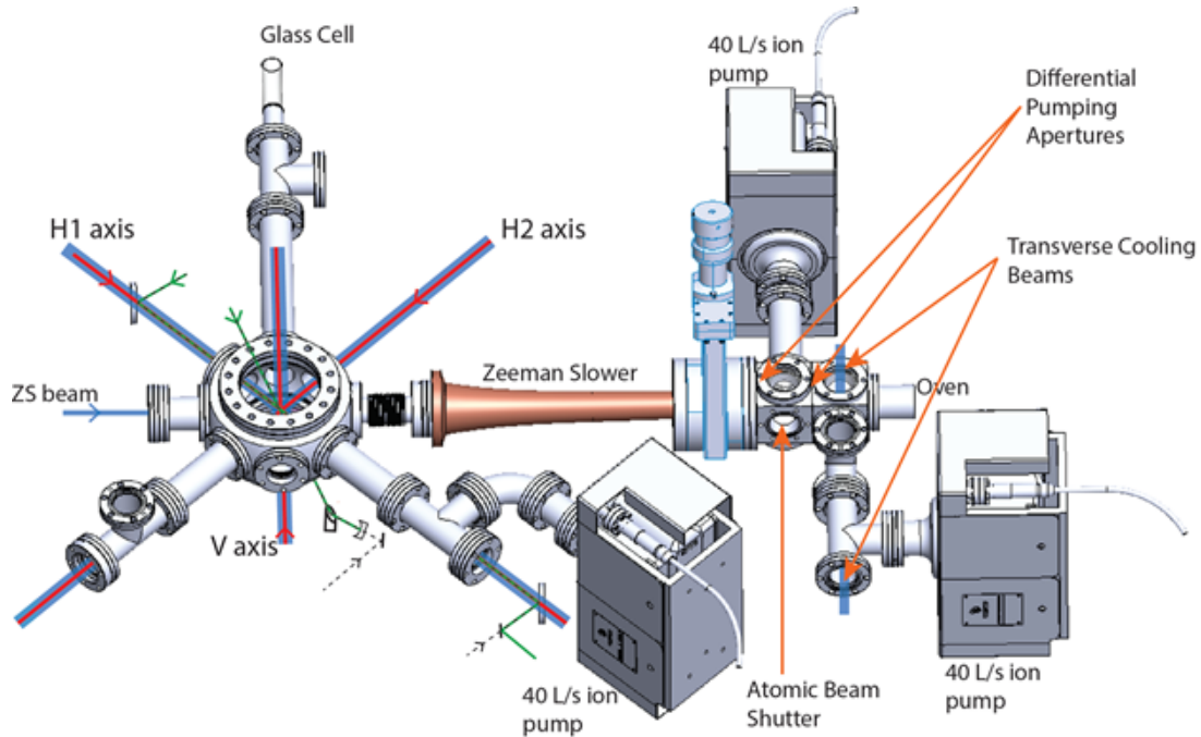
Figure 2.1: Vacuum chamber showing the position of the different laser beams. As the atomic beam exits the oven it is collimated using a stage of transverse cooling before being slowed using Zeeman slowing with a varying magnetic field and a counter-propagating laser beam. The atoms are captured at the center of the spherical octagon in a magneto-optical trap (MOT) based on the ^1S_0-^1P_1 transition before being transferred to a MOT based on the ^1S_0-^3P_1 transition for cooling to \mu\text{K} temperatures. The blue cooling light is shown in blue and the overlapped red cooling light and repumps are shown in red. The atoms are then usually transferred to a lattice, shown here in green, that is either Horizontal (H1 axis) or close to vertical (V axis). The atoms can then be probed with the clock laser, shown here as dashed lines, along the axis of the lattice. We also alternatively probe along the H2 axis to measure the radial temperature
