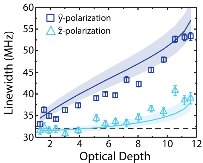
Figure 4.13: Linewidth broadening in the transverse direction \hat{z} using two orthogonal polarizations \hat{y} (blue, squares) and \hat{z} (cyan, triangles) which is classically forbidden.
