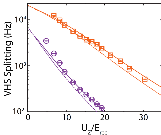
Figure 7.18: Carrier transition splitting for different lattice depths for the |g\rangle_0 \rightarrow |e\rangle_0 transition (purple, circles) and the |e\rangle_1 \rightarrow |g\rangle_1 transition (orange, squares). The splitting is extracted using fits from a convolution of a lorentzian lineshape and the density of states and the lattice depth is extracted from the sideband scan.
