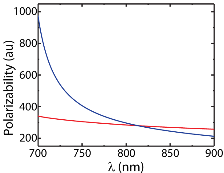
Figure 2.15: The scalar polarizability of the two different clock state ^1S_0 (red) and ^3P_0 (blue). The magic wavelength at 813 nm occurs when the polarizability of the two clock states are the same.
