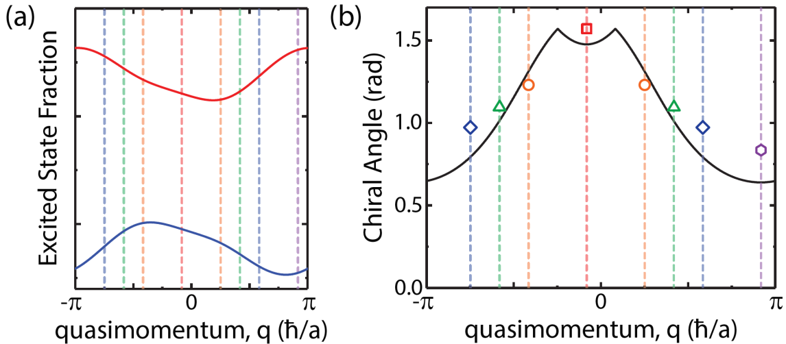
Figure 7.23: (a) Spin-orbit coupled band structure during the Rabi flopping, showing the q selection regions as dashed lines corresponding to the colors in Fig. 7.22. (b) The extracted Chiral angles for the different q -selections by fitting the data in Fig. 7.22. The black solid line is a theory fit using Eq. 7.26.
