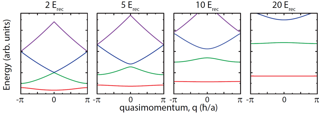
Figure 7.2: Lattice Band structure for increasing lattice depth. The four lowest bands are shown. The energy width of each band is proportional to the tunneling rate which increase with decreasing depth.
