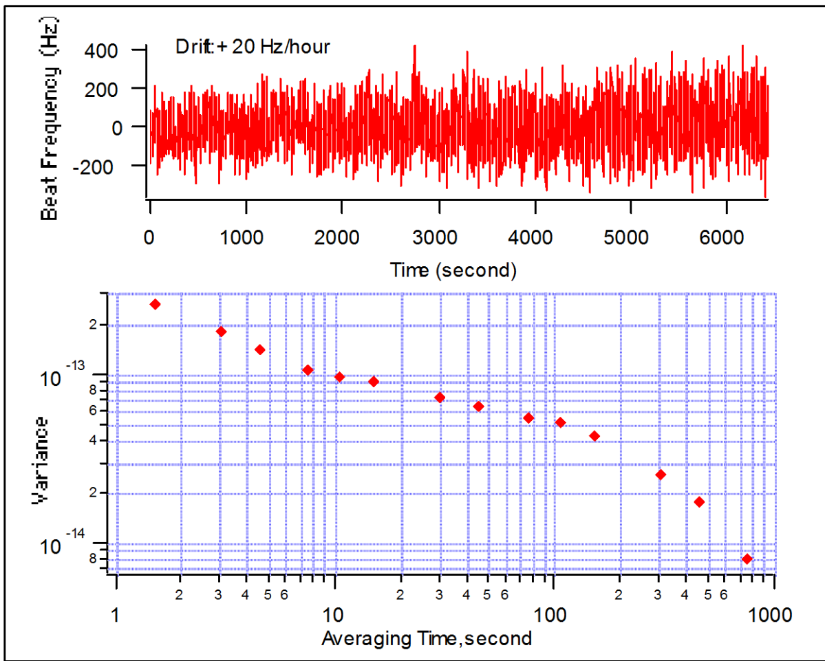
Figure 5 Time record of the beat frequency between two stabilized lasers and the Allan variance.
