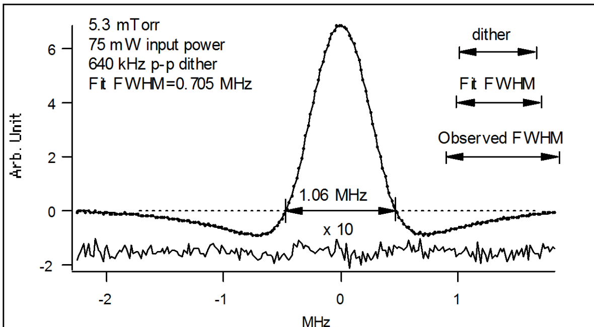
Figure 3 Frequency scan of the C_2HD ( v_2 + 3v_3 ) P(5) line and overlaid theoretical fit, with fit residuals magnified by 10 times.
