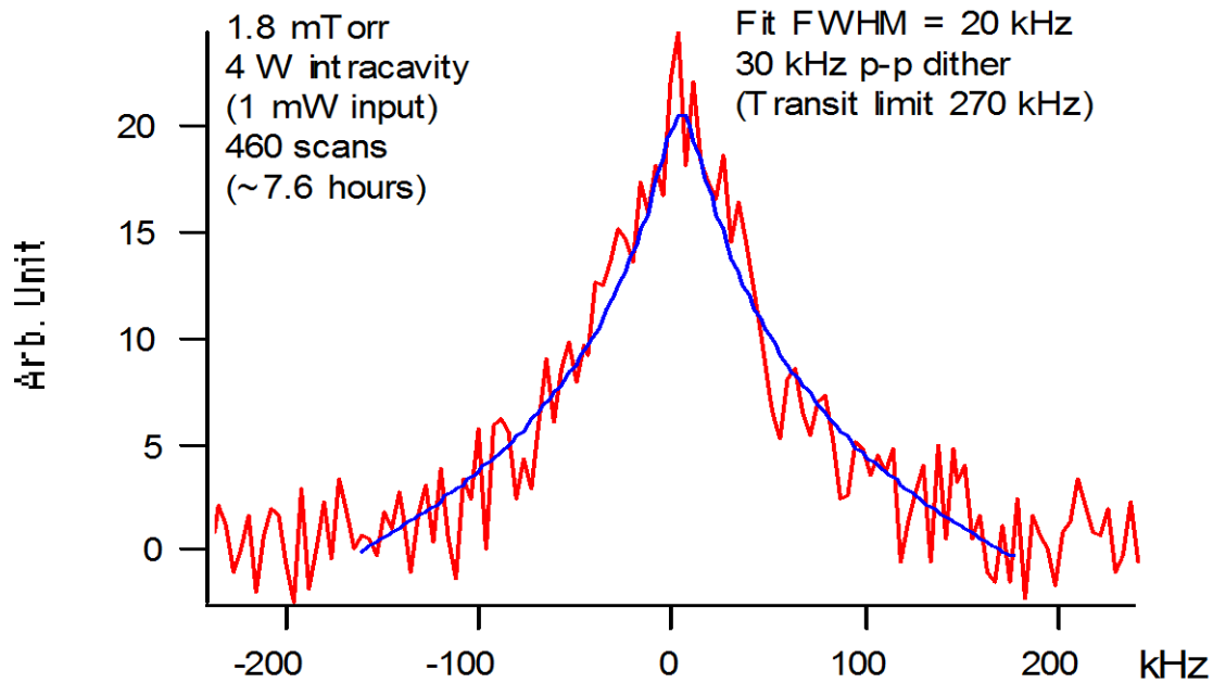
Figure 6 With low power and gas pressure, slow molecules give a linewidth 13 times below the transit limit.
