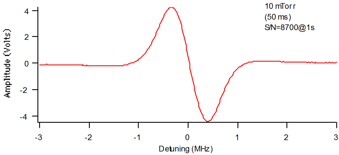
Figure 4 Molecular discrimination signal used for stabilizing Nd:YAG laser, obtained by the 2nd harmonic detection of the molecular dispersion.
