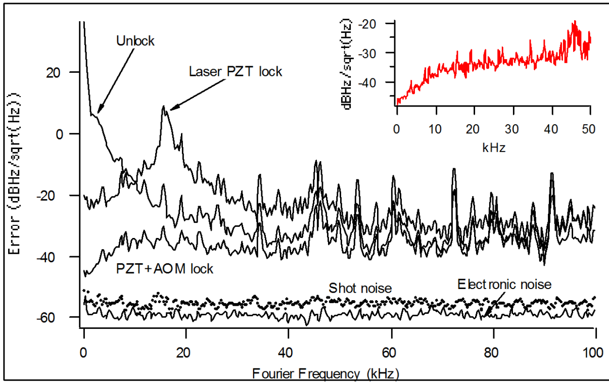
Figure 2 Laser/cavity locking frequency noise spectral density.
