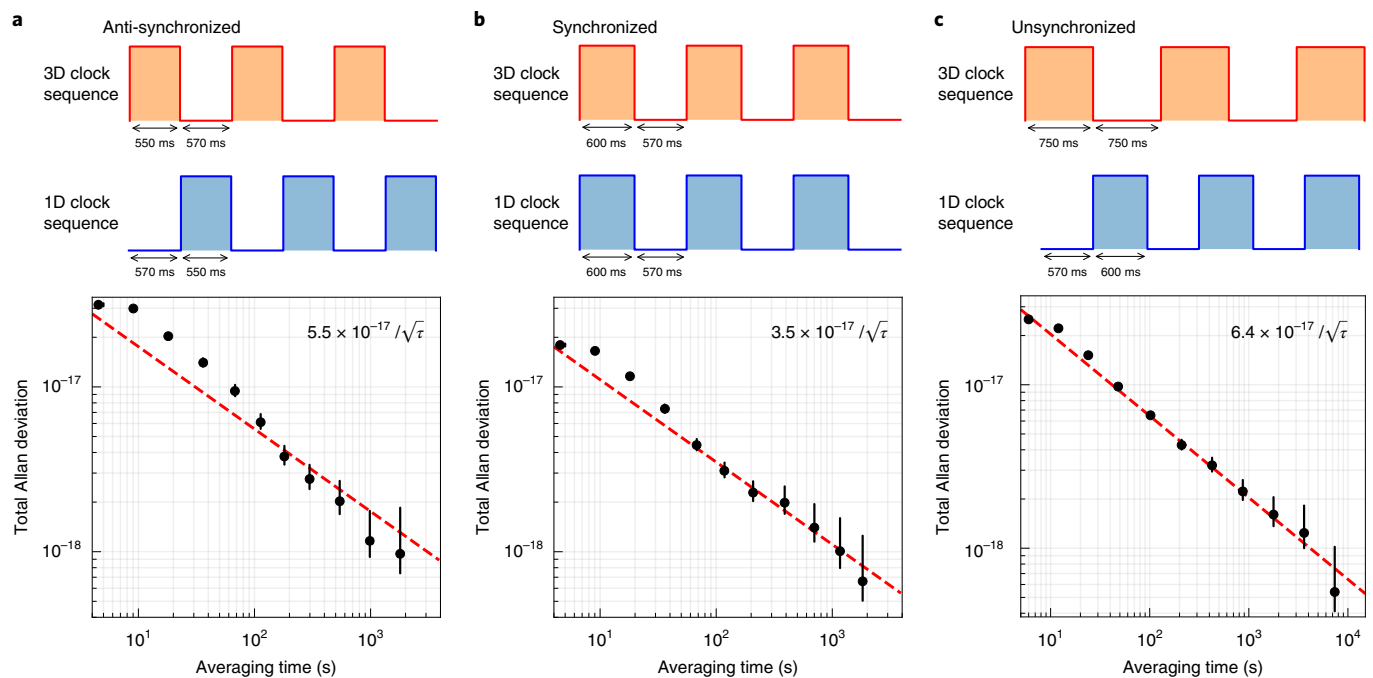
Fig. 5 | Stability comparison between 1D and 3D clocks. The total Allan deviation of the fractional measurement instability is reported as \frac{1}{\sqrt{2}}(v_{1D}(t) - v_{3D}(t))/\nu_c . Dashed red lines represent a weighted 1/\sqrt{\tau} fit to the data past 80 s and extend out to the full measurement time for each comparison. a , Anti-synchronous comparison. The two clocks are run with with the clock pulses anti-synchronized to prevent common mode rejection of the Dick effect. The observed instability of 5.5(3) \times 10^{-17}/\sqrt{\tau} along with a detailed noise model allow one to infer an instability of 4.8 \times 10^{-17}/\sqrt{\tau} for independent clock operation. b , Synchronous comparison. The two clock pulses are synchronized to provide maximal common mode rejection of the Dick effect. An instability of 3.5(2) \times 10^{-17}/\sqrt{\tau} , limited primarily by QPN, is observed. The final data point at 1,800 s reaches a value of 6.6 \times 10^{-19} . c , Unsynchronized comparison. This measurement demonstrates the capability of both clocks to average down with state-of-the-art stability for a comparison spanning several hours. An instability of 6.4(1) \times 10^{-17}/\sqrt{\tau} is observed. Error bars indicate 1\sigma confidence intervals.
