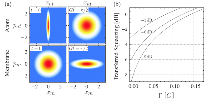
FIG. 2 (color online). (a) Wigner functions of atom and membrane (upper and lower panels, respectively). At t = 0 (left-hand panels) the atom is in a squeezed state (9 dB) and the membrane in a thermal state with a mean number of phonons \bar{n} = 5 . An exact solution of the equation of motion (2) with losses \Gamma = \Gamma_c, \Gamma_m, \Gamma_{at} at rate \Gamma = 0.1G shows that after a time Gt = \frac{\pi}{2} (right-hand panels) the states are exchanged, up to a trivial rotation in phase space by 90^\circ . (b) Squeezing transferred to membrane (maximized over time), versus loss rate \Gamma , for the indicated values of initial atomic position fluctuations.
