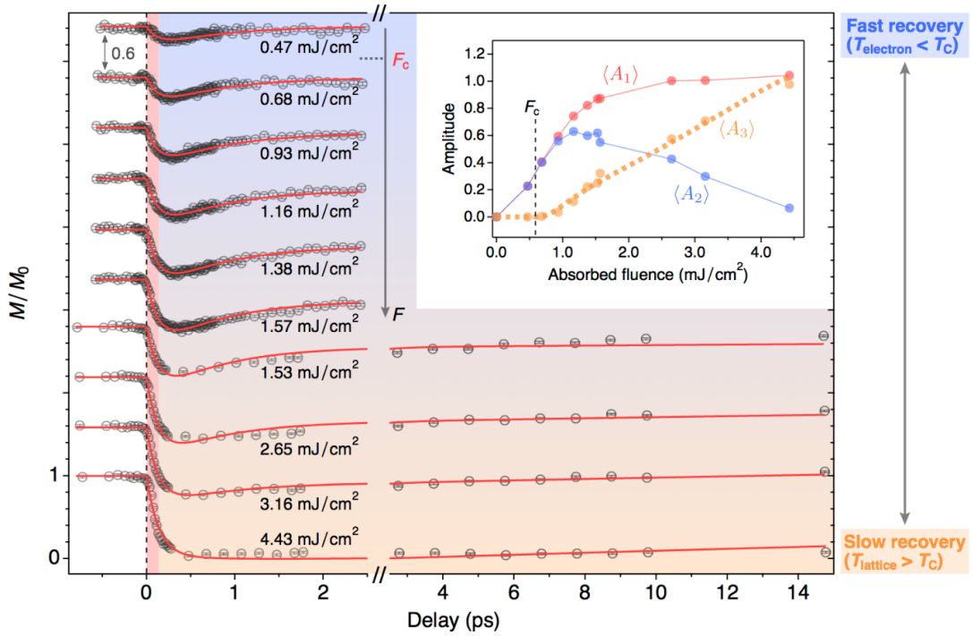
Figure 5.3: Magnetization dynamics in Ni measured using Tr-TMOKE over a full range of laser fluences. The highest fluence is sufficient to fully suppress the sample magnetization. The data are offset for clarity. Red curves: Fits to our microscopic model which considers the critical behavior, as well as the depth-average effects in the Tr-TMOKE measurements. Inset: Fluence-dependent amplitudes of the demagnetization and recovery processes directly extracted from the Tr-TMOKE results. In the Tr-TMOKE results, the magnetization \langle M \rangle and the extracted amplitudes \langle A_1 \rangle , \langle A_2 \rangle , and \langle A_3 \rangle are averaged over the entire probed depth. The dashed yellow line highlights the linear relation of the amplitude \langle A_3 \rangle to the absorbed fluence when the fluence is above the critical fluence.
