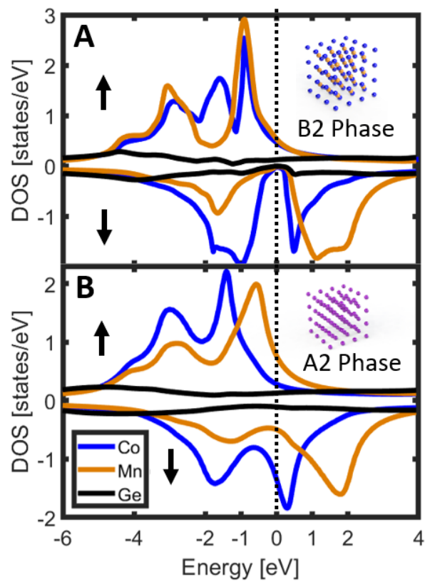
Figure 6.3: Density of states for Co 2 MnGe in the (A) B2 and (B) A2 phases. Note that the half-metallic character is only present in the B2 phase.
