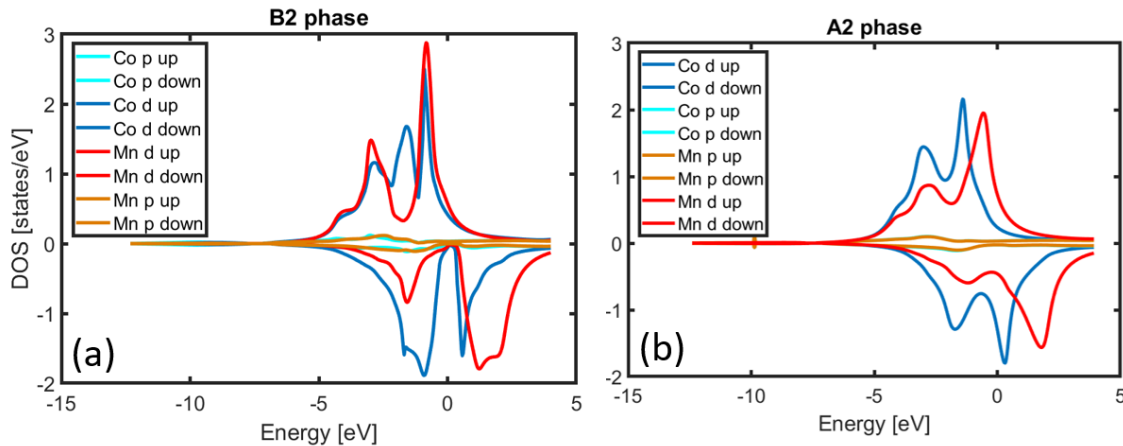
Figure B.5: Element and orbital specific DOS for (a) B2 and (b) A2 phases. Note that the p orbitals are an order of magnitude smaller than the d orbitals, however transitions take place from p to d or d to p orbitals.
