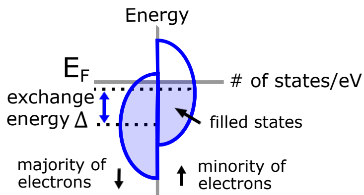
Figure 2.2: Stoner Model for ferromagnetic transition metals, and illustration of terms used for the description of this model. The filled electron states (at zero temperature) below the Fermi energy E_F are shaded. The spin population with greater occupied states is called the majority band, while the population with less occupied states is called the minority band. The centers of the two bands are separated by the exchange energy \Delta .
