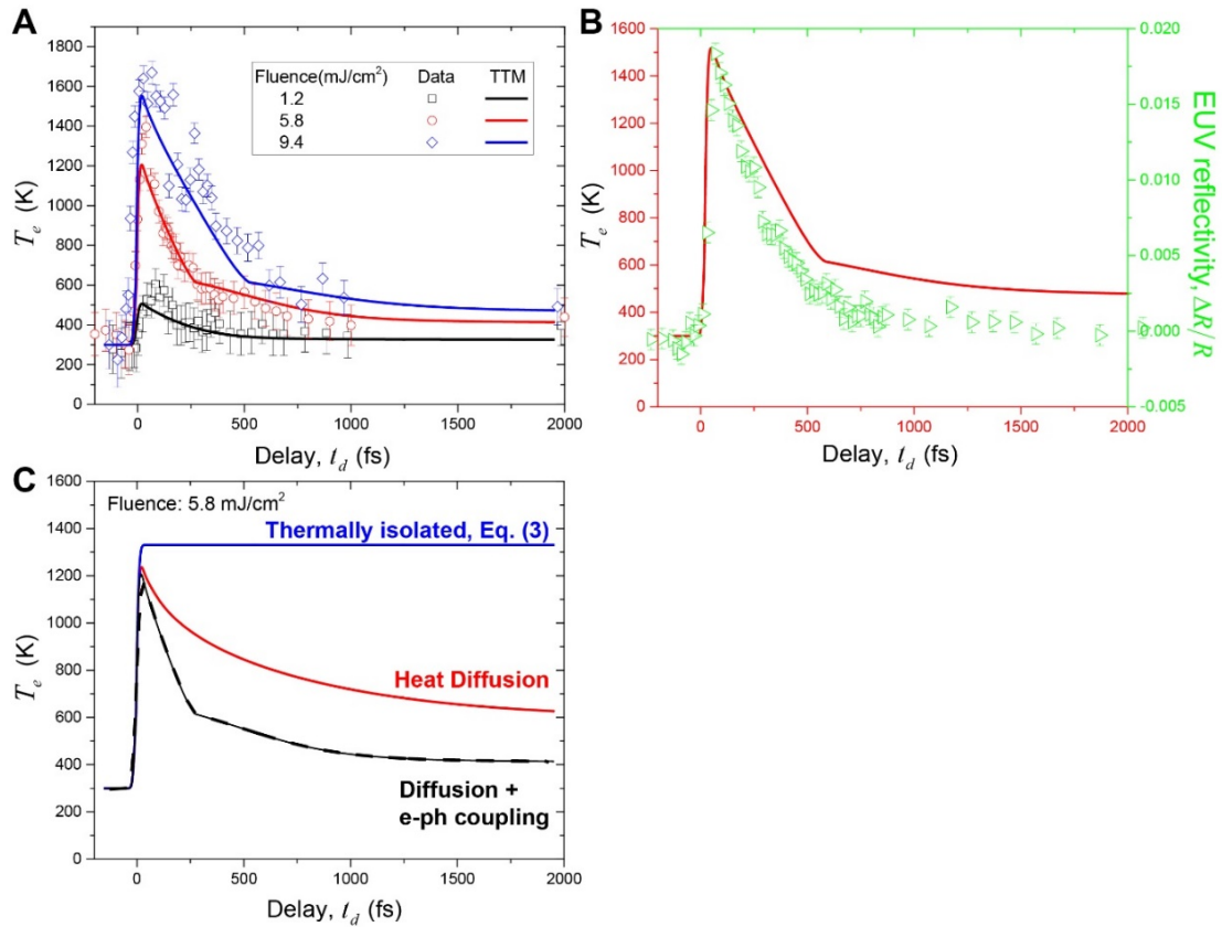
Figure 4.8: Two-temperature model. (A) The electron temperature measured using Tr-ARPES in comparison with the simulation results from TTM for the top 1nm thick layer of Ni with different pump fluence. (B) The transient EUV reflectivity results in comparison with the TTM simulation considering the average over a EUV probing depth of \approx 10 nm. (C) The electron temperature simulated by TTM considering the situations: 1) thermally isolated, same as Eq. 4.1; 2) only heat diffusion; 3) heat diffusion + e-ph coupling. The dashed line represents the simulation results convolved with the experimental time resolution.
