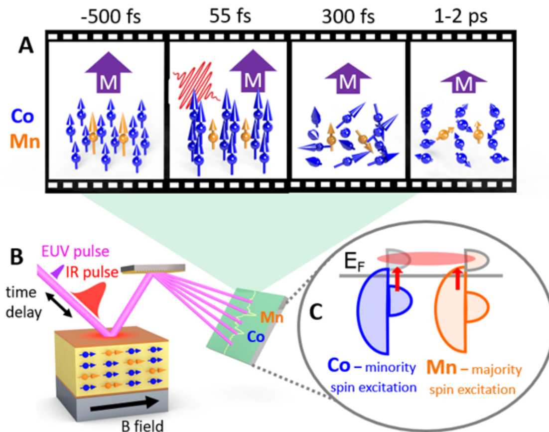
Figure 6.1: (A) Representation of spin dynamics in \text{Co}_2\text{MnGe} . Before excitation, Mn atoms (orange arrows) have a 3x larger magnetic moment than Co atoms (blue arrows), which are 2x more abundant in the bcc lattice. The purple arrow represents the net magnetic moment of the compound. Upon excitation, the Mn moment begins to decrease and the Co magnetic moment immediately grows by 10%. This occurs within the duration of the pump pulse. Hundreds of femtoseconds later, the Mn and Co atomic spins become disordered, and the angular momentum begins to transfer to the lattice. The net magnetic moment begins to decrease. After 1-2 ps, the spins have reached their maximum quenching. (B) Schematic of the experimental apparatus. Ultrafast femtosecond infrared pulses are used to excite the sample, while the magnetization dynamics are tracked with femtosecond EUV pulses recorded on a spectrometer. (C) Density of states for each element in the half metal. Note that the minority spin channel is gapped, with no available states at the Fermi level for the minority channel. Critically, this gap is larger for Mn than for Co. After excitation, the conduction band states are hybridized, as illustrated by the shared red wavefunction.
