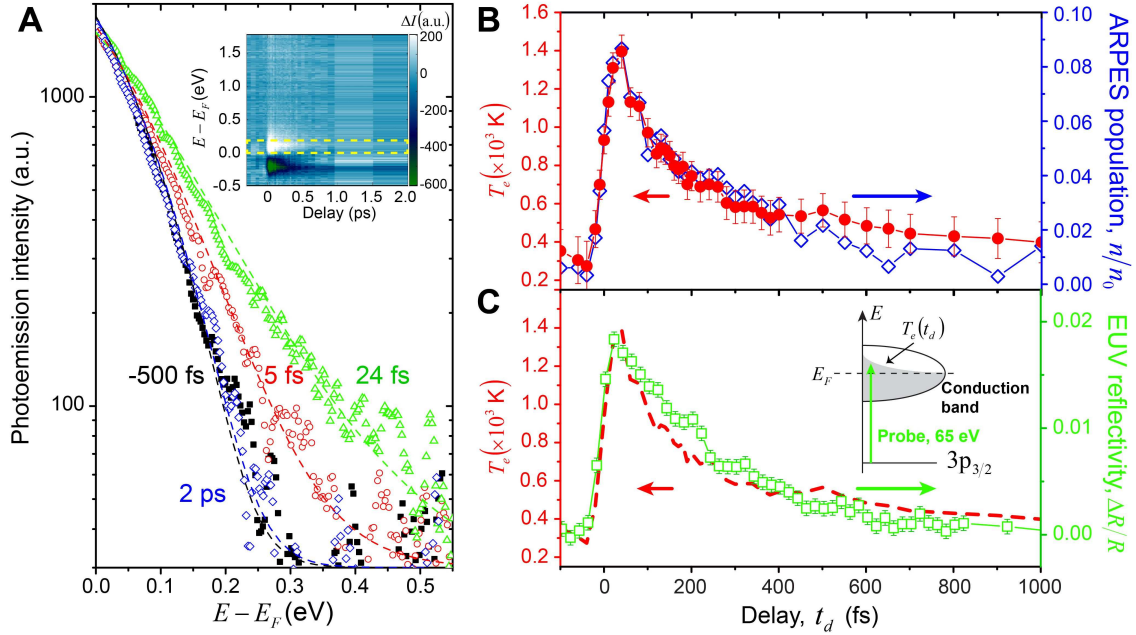
Figure 4.3: Ultrafast charge dynamics in Ni. (A) Log plots of the photoemission intensity above E_F for F \approx 6 \text{ mJ/cm}^2 and at different t_d , integrated from k \approx 0.85 \text{ \AA}^{-1} to k \approx 1.3 \text{ \AA}^{-1} in the momentum space. The dashed lines represent the fitting of the photoemission intensities with the Fermi-Dirac distribution convolved with experimental energy resolution (see appendix A). Inset: Integrated photoemission intensity as a function of pump-probe time delay. The yellow dashed box illustrates the integration region of electron population in (B). (B) Dynamics of the electron temperature and the relative electron population ( n/n_0 ) within 0.2 eV above E_F as a function of t_d . The electron population is normalized to the band electron population ( n_0 ) 0.2 eV below E_F (see appendix A). (C) Comparison of the electron temperature [red dashed line, same as (B)] and the change of EUV transient reflectivity at a similar pump fluence. Inset: EUV transient reflectivity measurement. The resonant EUV light (65 eV) directly probes the charge dynamics around E_F induced by the laser pump pulse. This measurement is averaged over k-space
