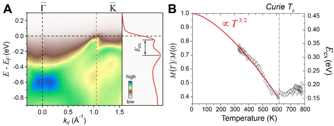
Figure A.5: Collapse of exchange splitting at the Curie temperature. (A) Static photoemission spectrum excited by He I \alpha photons ( h\nu = 21.218 \text{ eV} ) at the room temperature. Right panel: Energy distribution curve extracted at the momentum where the red dashed line is located. The exchange splitting ( E_{ex} ) can be clearly extracted using fitting procedure described in the previous section. (B) E_{ex} change reduces as the sample temperature increases.
