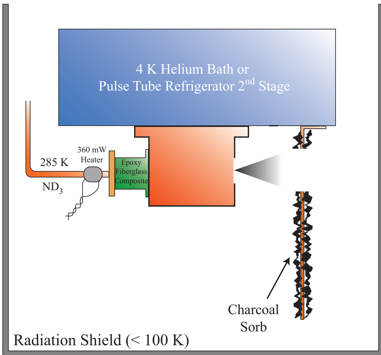
Figure 3.5: Illustration of our buffer gas beam assembly. The ND 3 gas is fed down a heated copper tube at 285 K. This hot supply tube is thermally isolated from the cold buffer gas cell via a polyetherimide (Ultem) insert and thin-walled epoxy-fiberglass composite (G10) tube. The pre-cooled He gas (not shown) is fed into the side of the cell. Charcoal sorb glued to copper plates ( \sim 2000 \text{ cm}^2 total) acts as a vacuum pump for He and ND 3 gas.
