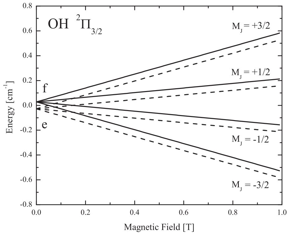
Figure 2.10: Zeeman shift of the {}^2\Pi_{3/2} ground state of OH. Since the Zeeman Hamiltonian only couples states of like parity, the two \Lambda -doublet levels of OH show exactly the same field dependence. Also, the lack of coupling between e and f states causes only diabatic level crossings.
