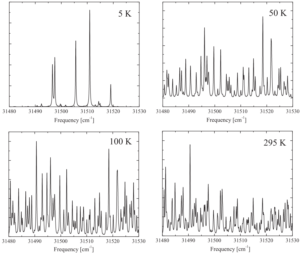
Figure 2.6: Simulated 2+1 REMPI spectrum of 2_0^5 rotational transitions in \text{ND}_3 . The simulated rotational temperature is given for each plot. For consistency of presentation, a Lorentzian width of 0.3 \text{ cm}^{-1} has been assumed for all spectral lines. Note that at high temperatures ( \gtrsim 100 \text{ K} ), Doppler broadening necessitates application of a Voigt lineshape to correctly fit experimental spectra.
