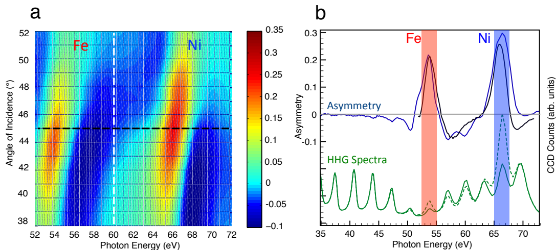
Figure 6.5: (a) Asymmetry spectra as a function of the angle of incidents. The spectra are measured from BESSY synchrotron (data courtesy from P. Grychtol, R. Adam and C. M. Schneider, Forschungszentrum Jülich, Germany) (b) The synchrotron asymmetry data at 45^\circ (black line) is compared with an asymmetry by use of the high-harmonic source (blue line). Both results are in agreement (top). The figure also displays high-harmonic spectra reflected from a Permalloy grating before (green line) and after (dashed green line) reversing the magnetization (bottom).
