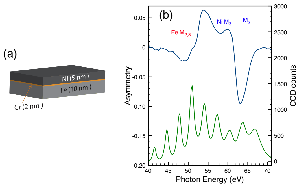
Figure 6.10: (a) The geometry of a magnetic trilayer of Fe, Cr and Ni. (b) The asymmetry measured from this sample is dominated by the top layer (Ni), while we only observe a weak signal for Fe.
