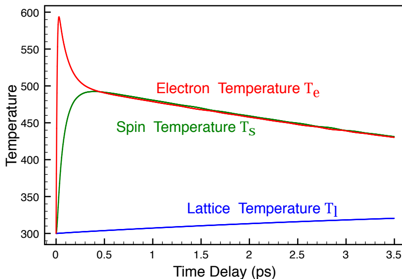
Figure 8.7: Simulation results for temperatures of electron, lattice and spin in nickel after an excitation by a 2.25 \text{ mJ/cm}^2 pump pulse. The demagnetization dynamics are a consequence from the temperature rise of the spin system.
