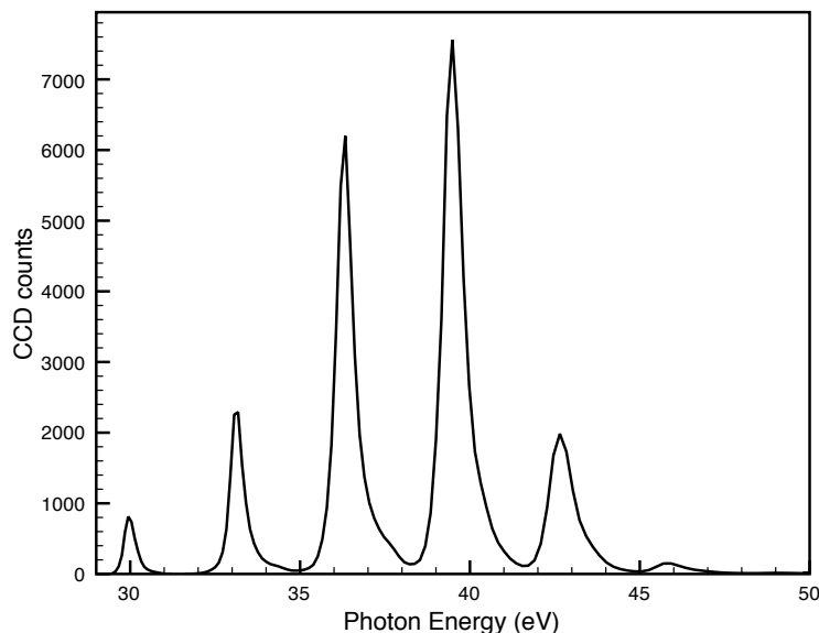
Figure 6.4: A typical high-harmonic spectrum using argon as the nonlinear medium and reflecting from a Permalloy grating with s-polarized light using an exposure time of 0.1 s.
