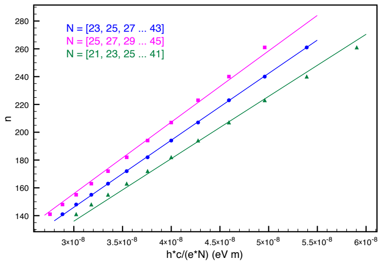
Figure 6.2: Determination of the correct high-harmonic orders. The diffracted distance ( n , in pixel) measured from the CCD image is plotted as function of the inverse high-harmonic order ( N scaled with \frac{e}{hc} ) from three series of high-harmonic orders. The series N = 23, 25, 27, \dots, 43 (blue) is the correct high-harmonic order since it gives the best fitting.
