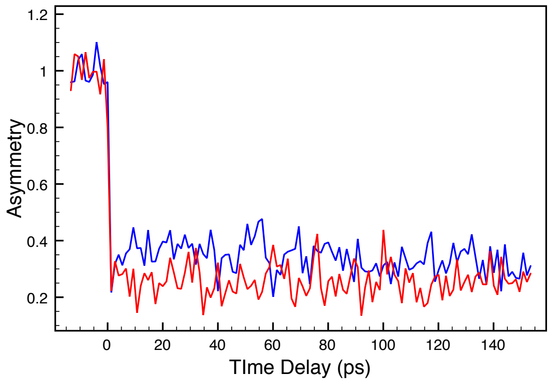
Figure 7.5: The long time scan of the asymmetry dynamics (up to 150 ps) of Permalloy-Copper.
