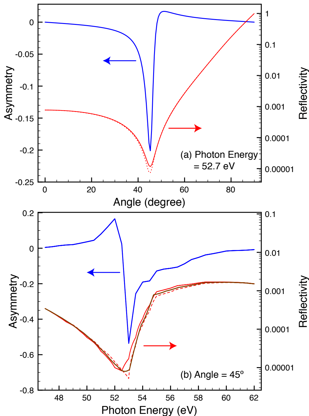
Figure 3.7: (Top) Asymmetry of Fe (blue) as function of incident angle at the photon energy of 52.7 eV ( M_{2,3} edges). Maximum asymmetry of 20% is close to the Brewster angle near 45^\circ when the reflectivity (red) is at the minimum. Both reflectivities after switching magnetization are shown as line and dashed line. (Bottom) Asymmetry of Fe as a function of photon energy near M-edges. The reflectivity calculated from an x-ray database [13] is also plotted (brown) to show the non-magnetic contribution.
