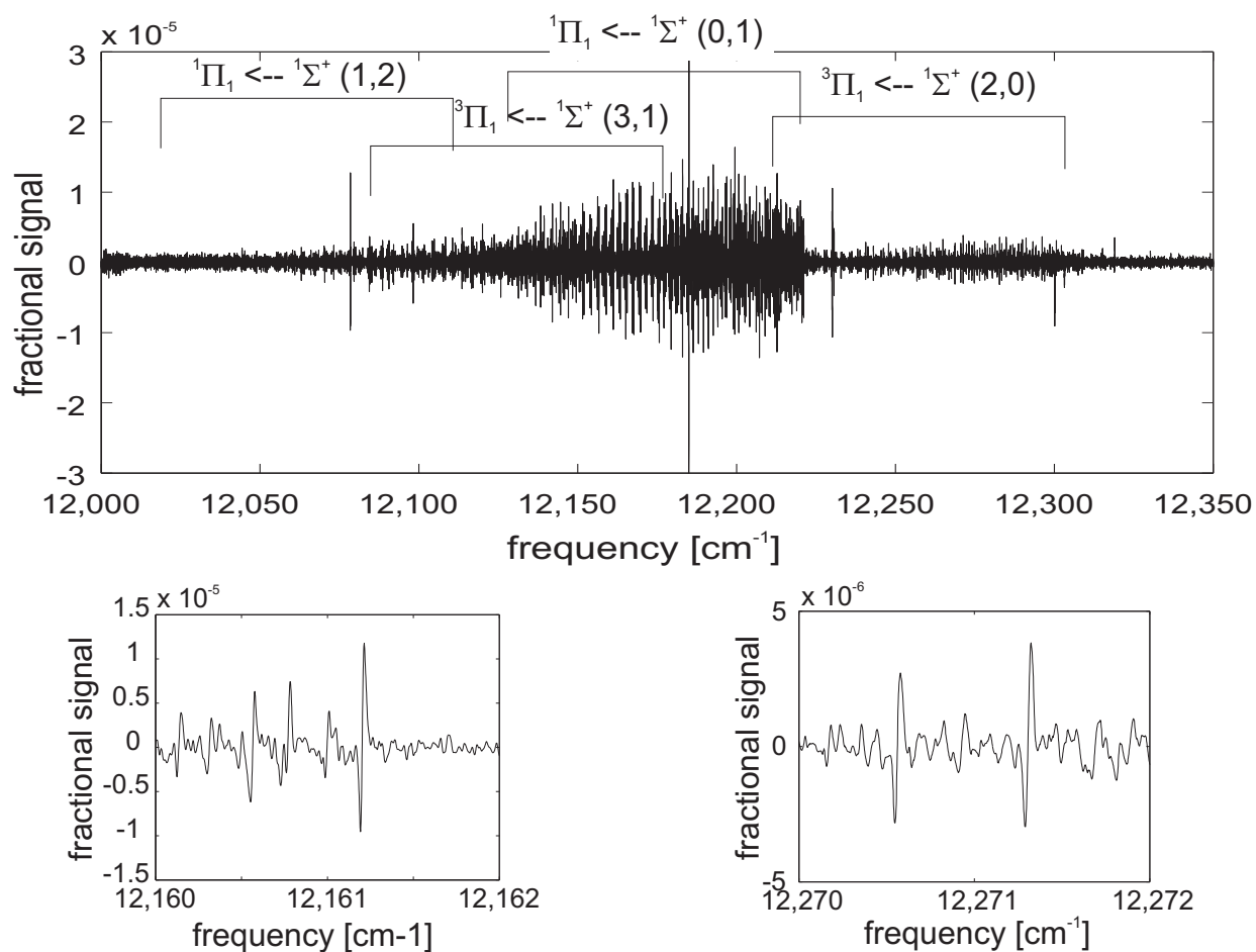
Figure 4.14: Region of spectrum with \text{HfF}^+ lines with smaller regions showing the characteristic velocity-modulation lineshape. Fits to the bands identified are discussed in Chapter Five. In the lower plots, the structure surrounding the strongest lines is due to additional \text{HfF}^+ molecular absorption. The fractional sensitivity measured without \text{HfF}^+ present is 3 \times 10^{-7} .
