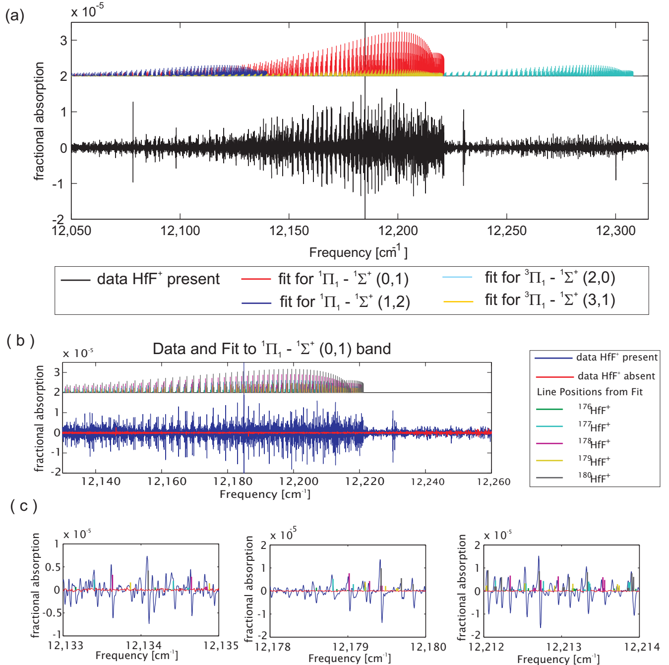
Figure 5.1: (a) Data and fits to the four \text{HfF}^+ bands identified with frequency comb velocity-modulation spectroscopy. Linestrengths for the fit positions are scaled by isotopic abundance, by an approximate rotational temperature of \sim 640 K, and by an overall transition strength to match the measured fractional absorption. (b) Region of the recorded spectra containing the {}^1\Pi_1 - {}^1\Sigma^+(0,1) band as well as at least three other \text{HfF}^+ bands with the fit for the {}^1\Pi_1 - {}^1\Sigma^+(0,1) band offset for clarity. (c) All five isotopes of \text{HfF}^+ are present and resolved for transitions with \Delta v \neq 0 . The additional structure with \text{HfF}^+ present (blue) consists of lines belonging to the other \text{HfF}^+ bands while the red line ( \text{HfF}^+ absent) shows the level of sensitivity of the system in this region.
