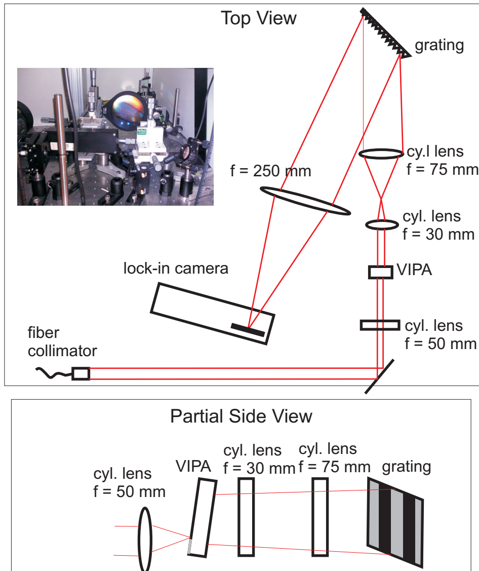
Figure 4.4: Schematic of imaging system. The VIPA provides high resolution, 1 GHz, but low free spectral range, 100 GHz. The grating resolves the 100 GHz FSR of the VIPA. The first f = 50 mm cylindrical lens focuses the light into the VIPA at the junction of the anti-reflective and high reflectivity coatings. After the VIPA, the cylindrical telescope expands the beam to fill the grating. The f=250 mm imaging lens then maps the differences in wavevector to differences in position at the detector plane of the camera. The inset shows a picture of the actual optics.
