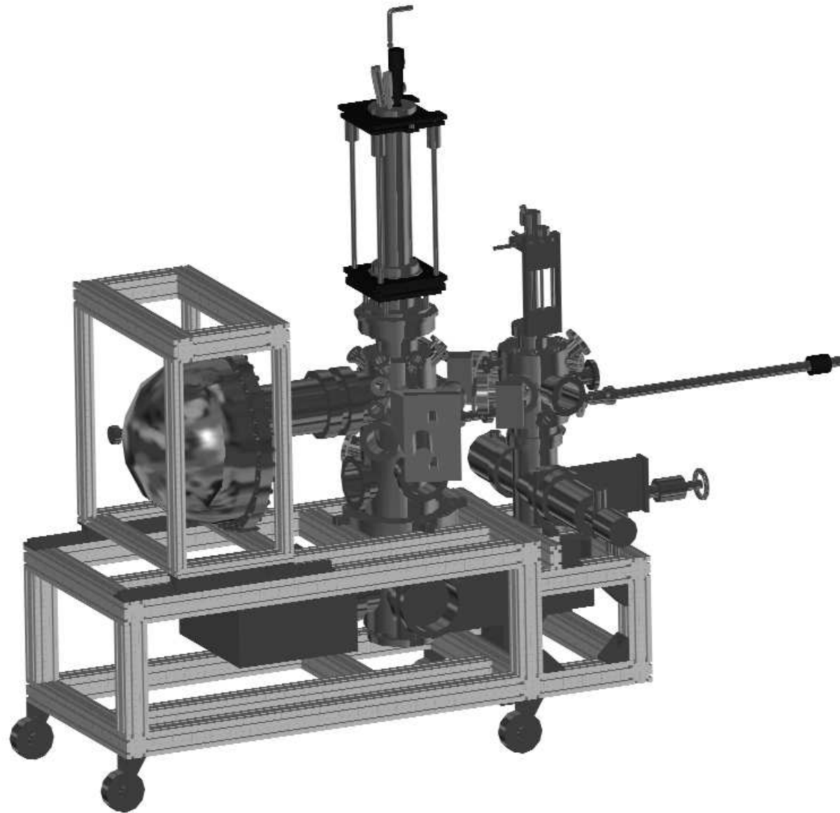
Figure C.2: CAD rendering 2 of the laser ARPES chamber. a
