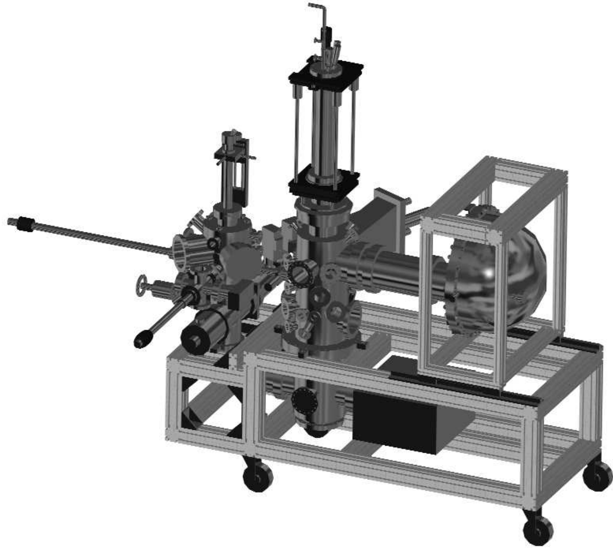
Figure C.1: CAD rendering 1 of the laser ARPES chamber. a
